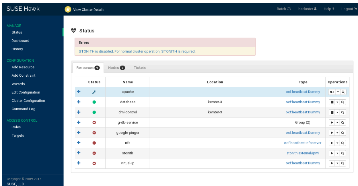
FIGURE 6.15: HAWK2—CLUSTER STATUS
