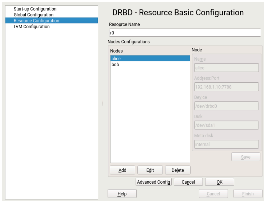
FIGURE 18.2: RESOURCE CONFIGURATION
