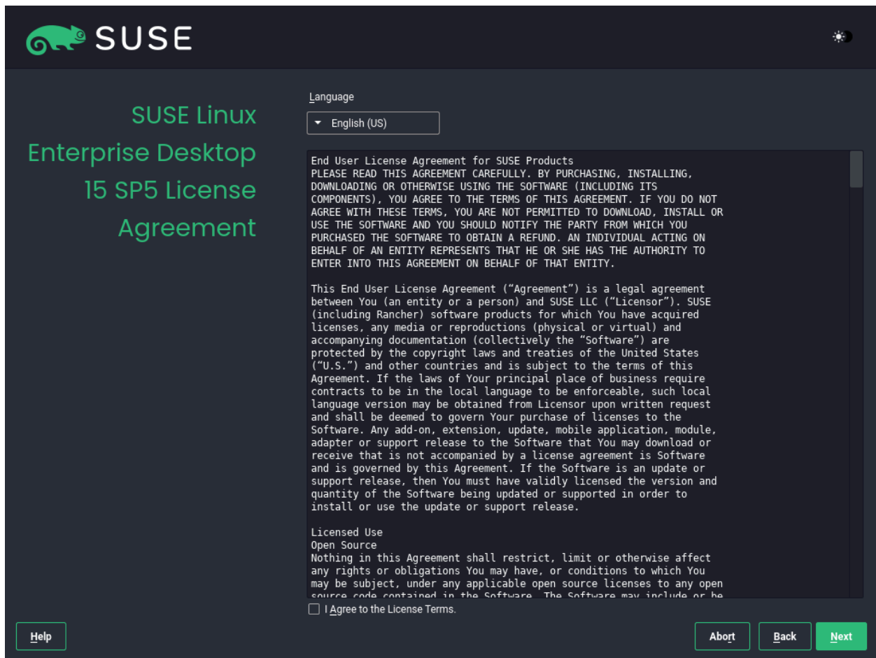
FIGURE 4.2: LICENSE AGREEMENT
