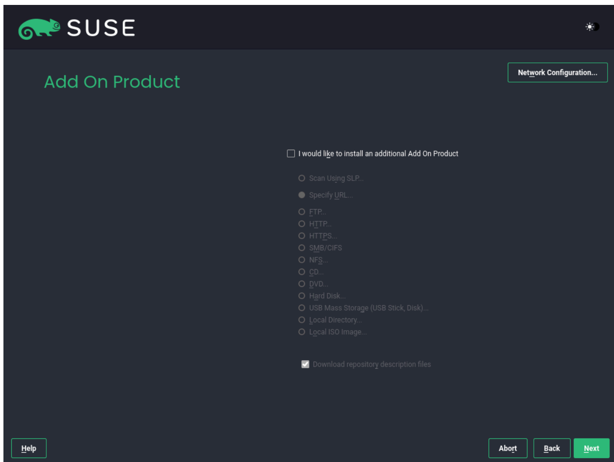
FIGURE 4.7: ADD-ON PRODUCT
