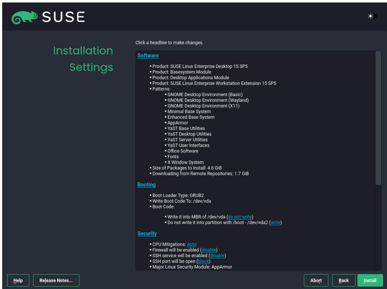
FIGURE 4.13: INSTALLATION SETTINGS
