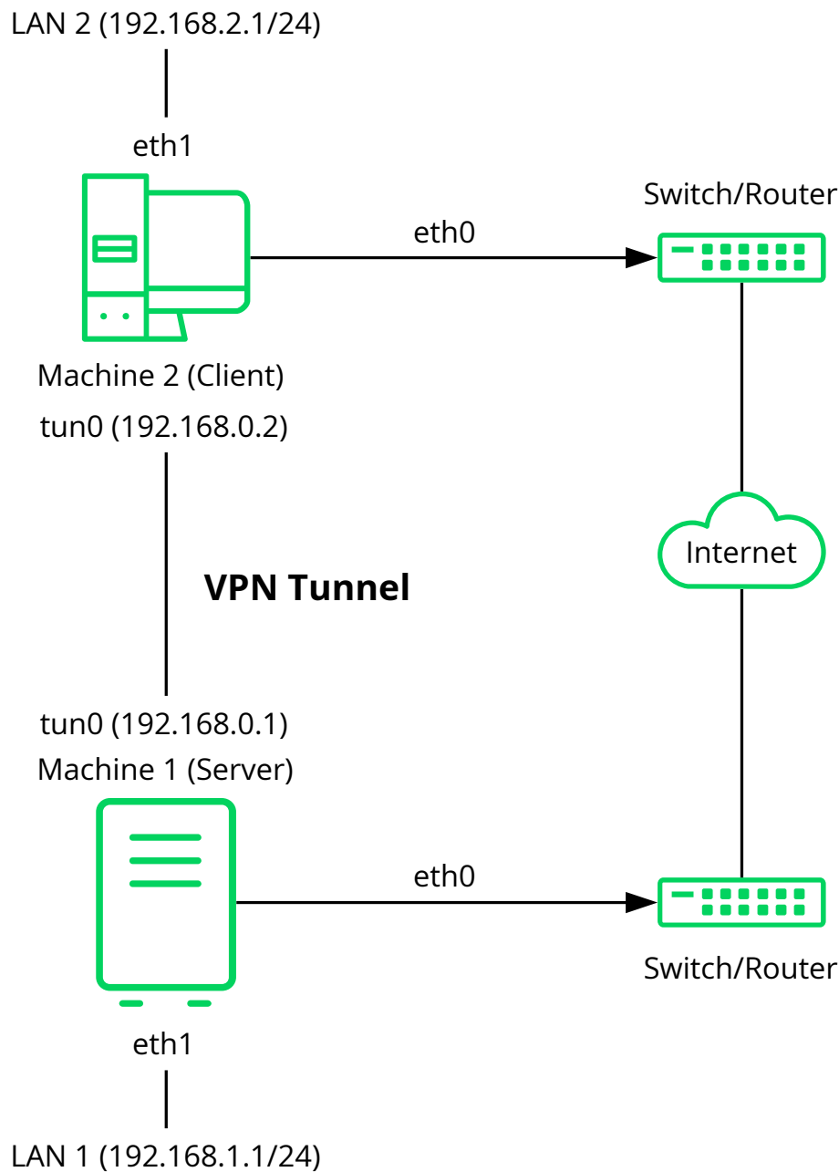
FIGURE 17.1: Routed VPN
