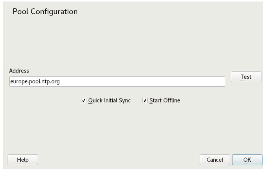
FIGURE 30.2: ADDING A TIME SERVER
