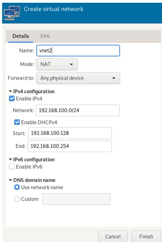
FIGURE 12.3: CREATE VIRTUAL NETWORK
