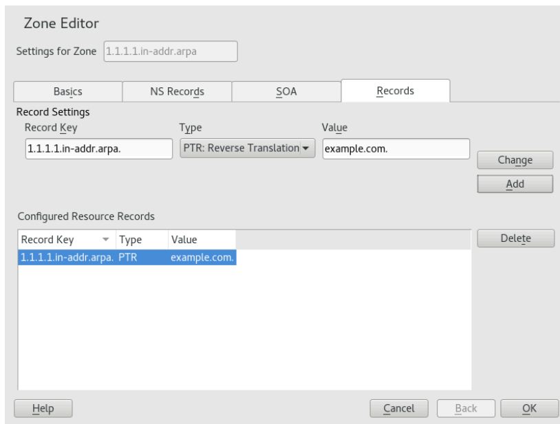
FIGURE 31.11: ADDING A REVERSE RECORD
