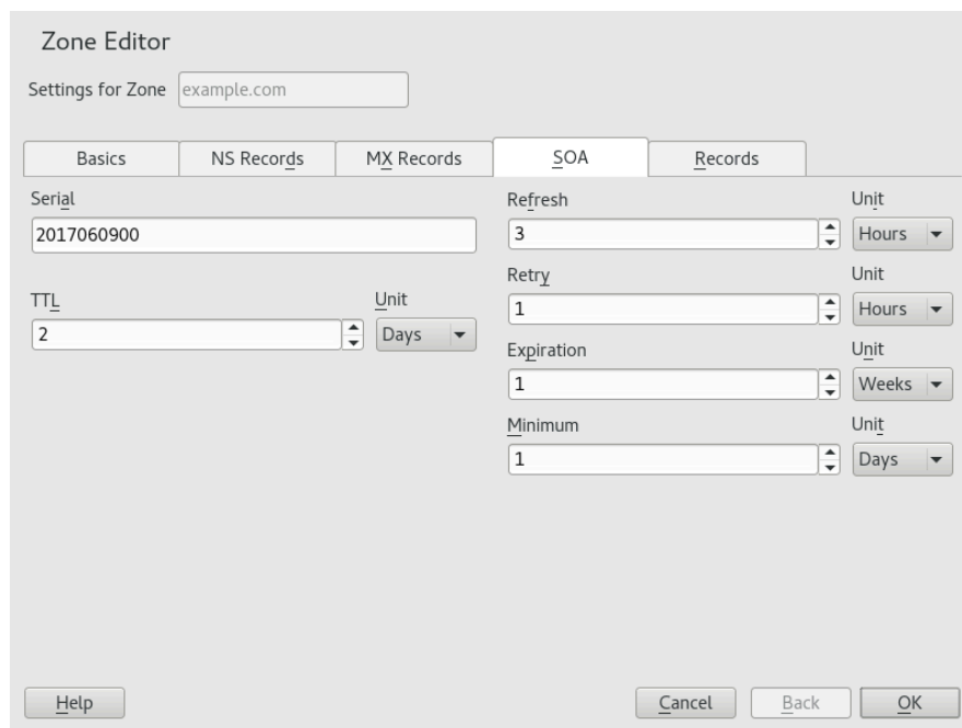
FIGURE 31.8: DNS SERVER: ZONE EDITOR (SOA)
