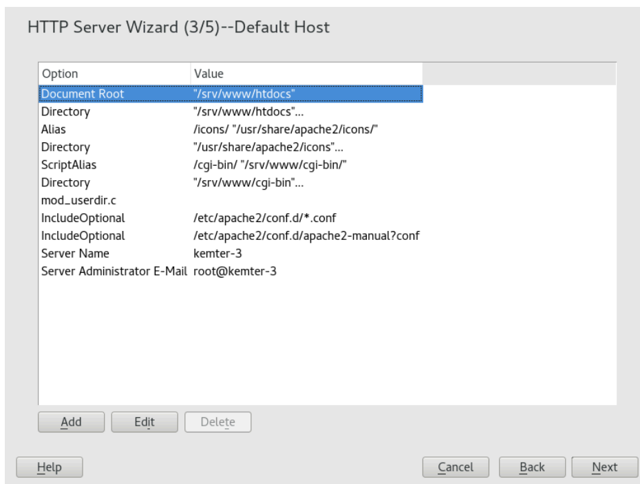
FIGURE 34.1: HTTP SERVER WIZARD: DEFAULT HOST
