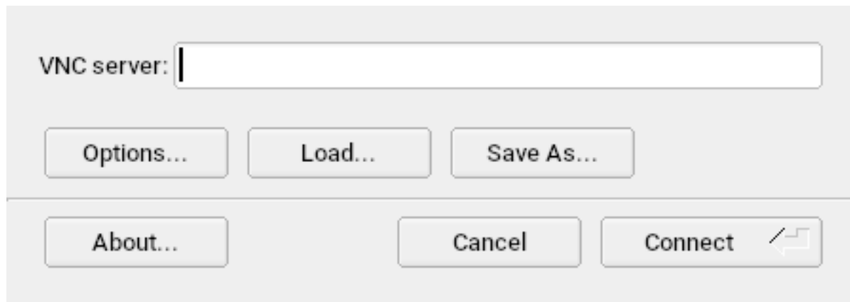
FIGURE 10.1: VNCVIEWER
