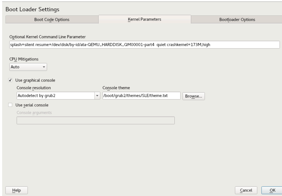
FIGURE 14.5: KERNEL PARAMETERS
