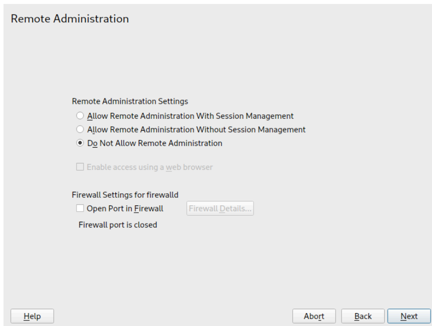
FIGURE 10.7: REMOTE ADMINISTRATION
