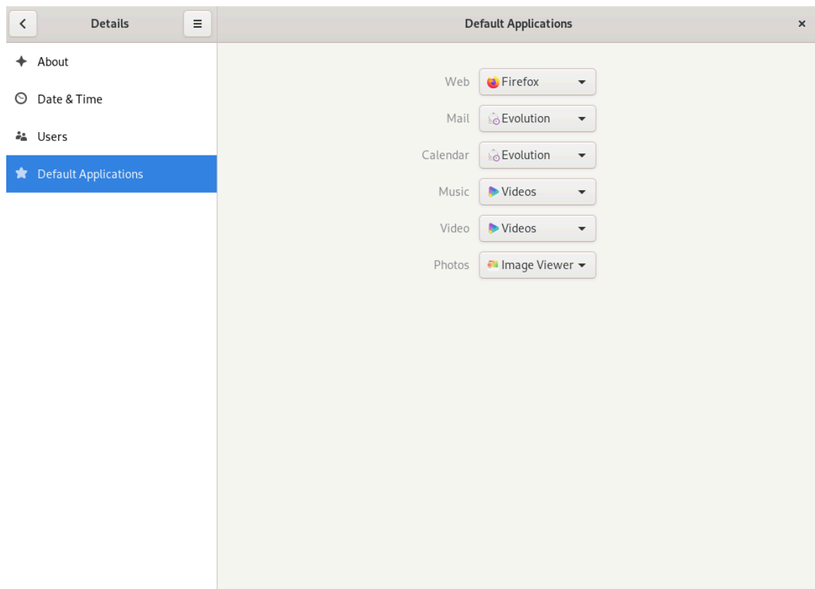
FIGURE 3.7: DEFAULT APPLICATIONS
