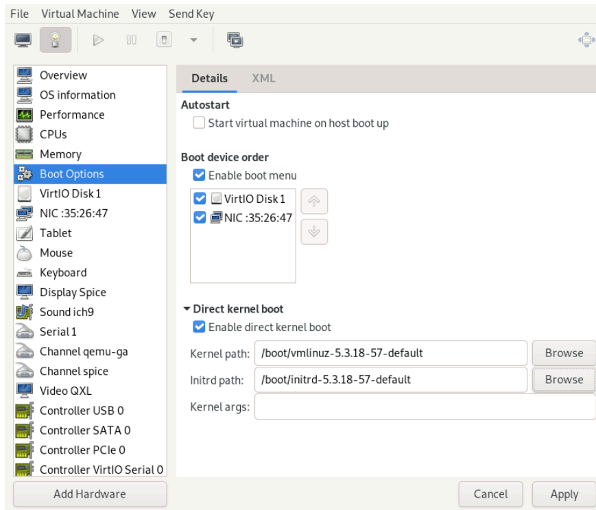
FIGURE 14.8: BOOT OPTIONS
