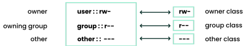
FIGURE 19.1: MINIMUM ACL: ACL ENTRIES COMPARED TO PERMISSION BITS
