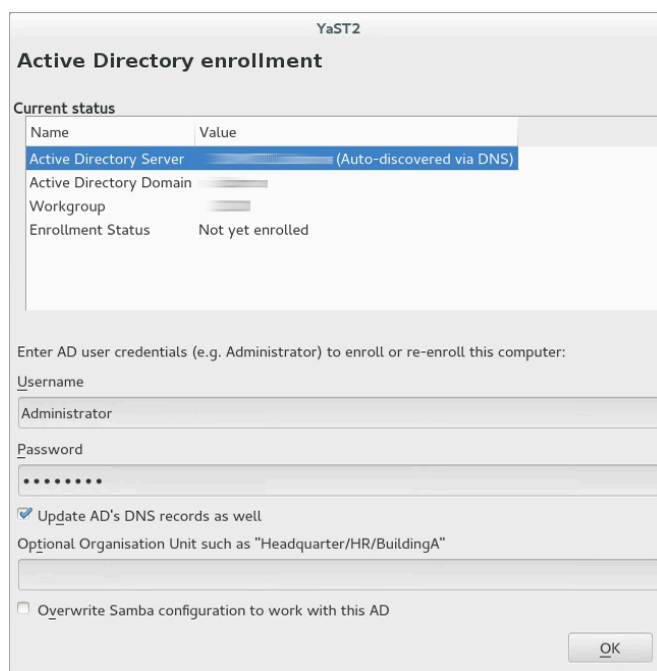
FIGURE 7.3: ENROLLING INTO A DOMAIN
