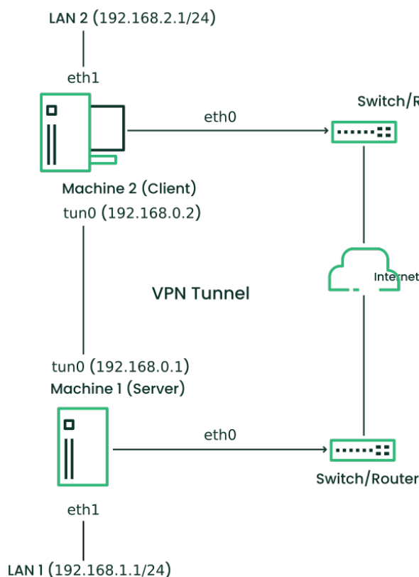
FIGURE 24.1: ROUTED VPN
