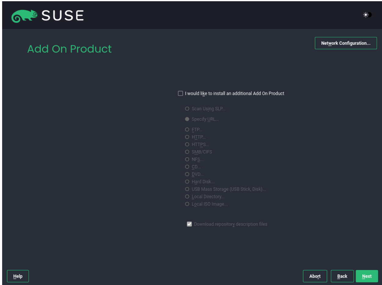
FIGURE 9.10: ADD-ON PRODUCT
