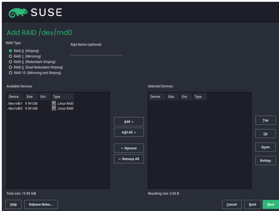
FIGURE 11.5: RAID PARTITIONS
