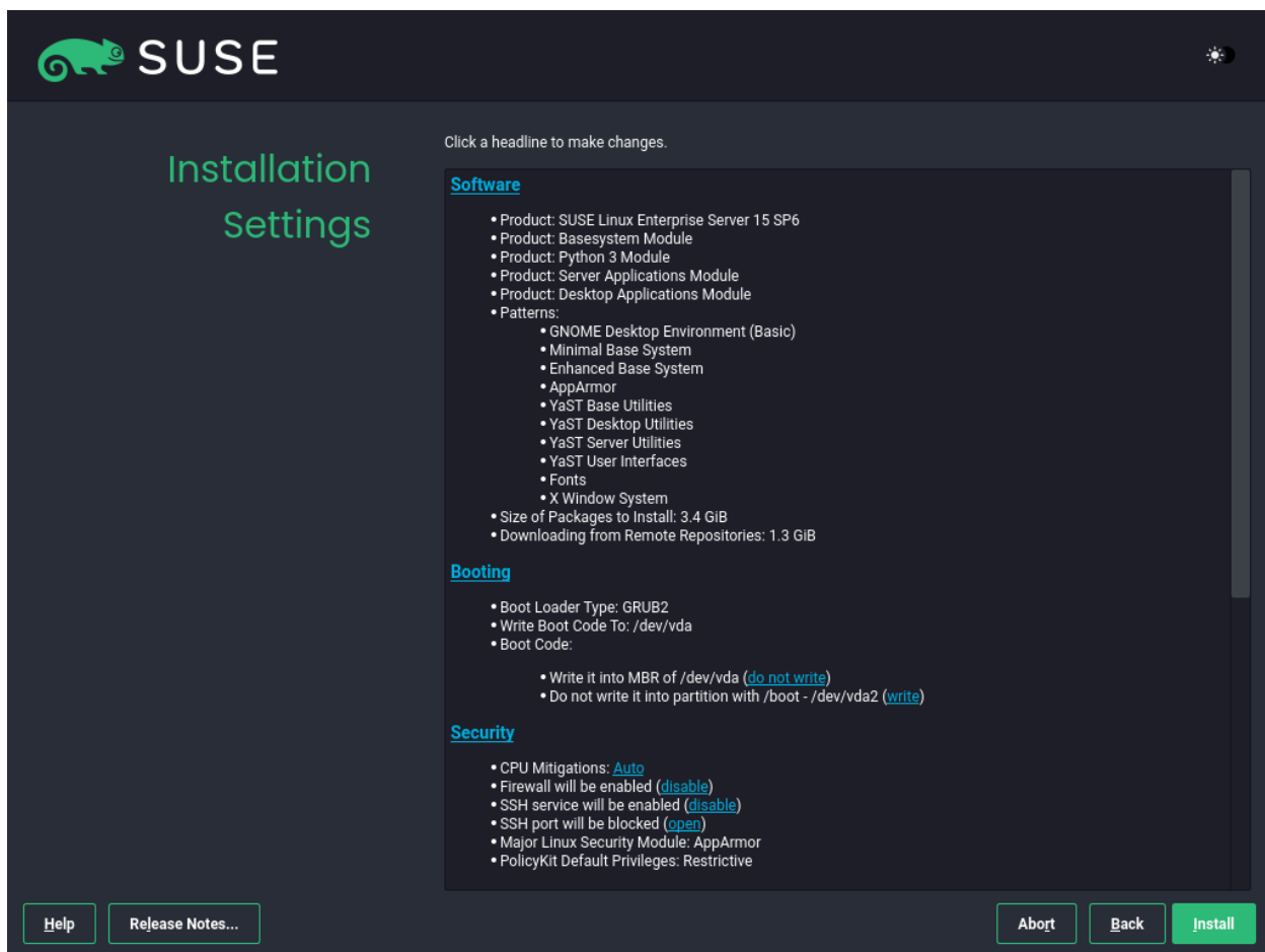
FIGURE 9.16: INSTALLATION SETTINGS
