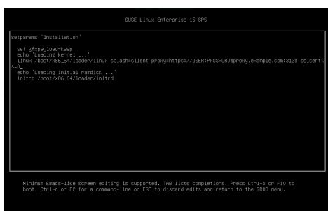
FIGURE 8.3: GRUB OPTIONS EDITOR
