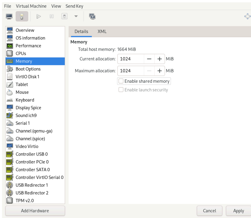
FIGURE 14.7: MEMORY VIEW
