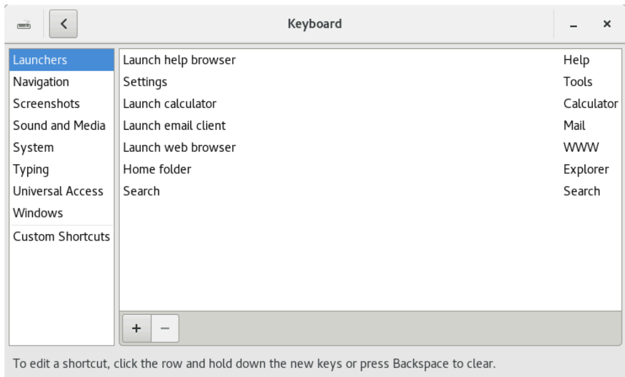
FIGURE 3.2: KEYBOARD DIALOG
