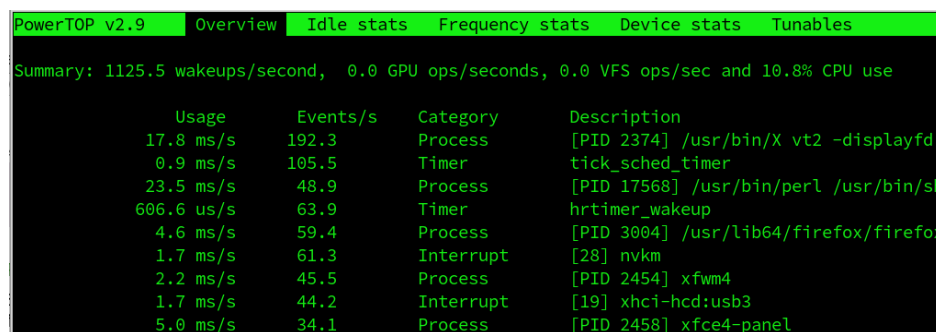
FIGURE 12.1: POWERTOP IN INTERACTIVE MODE
