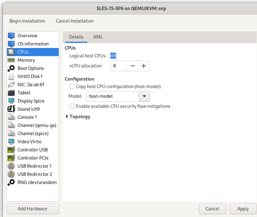
FIGURE 16.5: THE DETAILS VIEW OF VIRTUAL MACHINE CONFIGURATION
