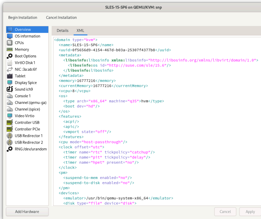
FIGURE 16.2: XML VIEW OF VIRTUAL MACHINE CONFIGURATION
