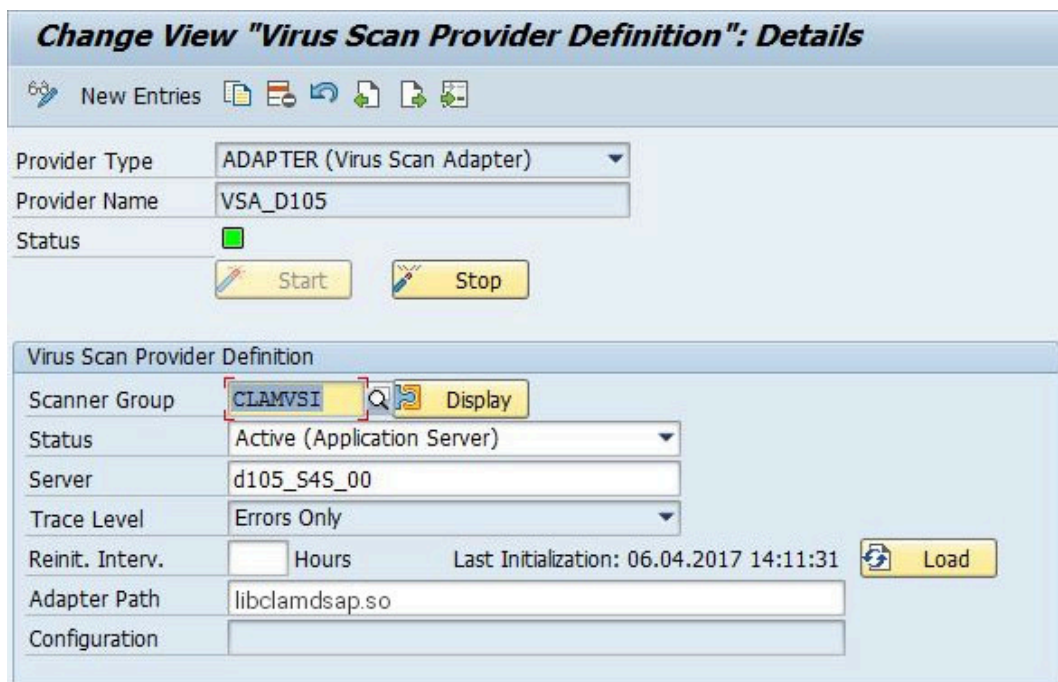
FIGURE 12.3: CHANGE VIEW "VIRUS SCAN PROVIDER DEFINITION"
